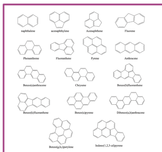
Figure 10: Molecular structures of the most common PAHS (Hussain 2018)
